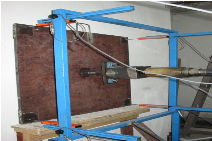
Figure 12. The location of loading plate and LVDTs.
