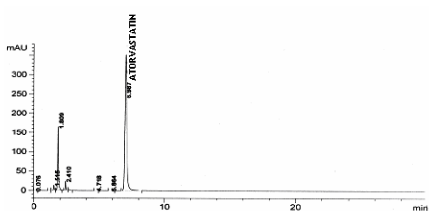
Figure 4. The chromatogram of alkali degraded sample.
