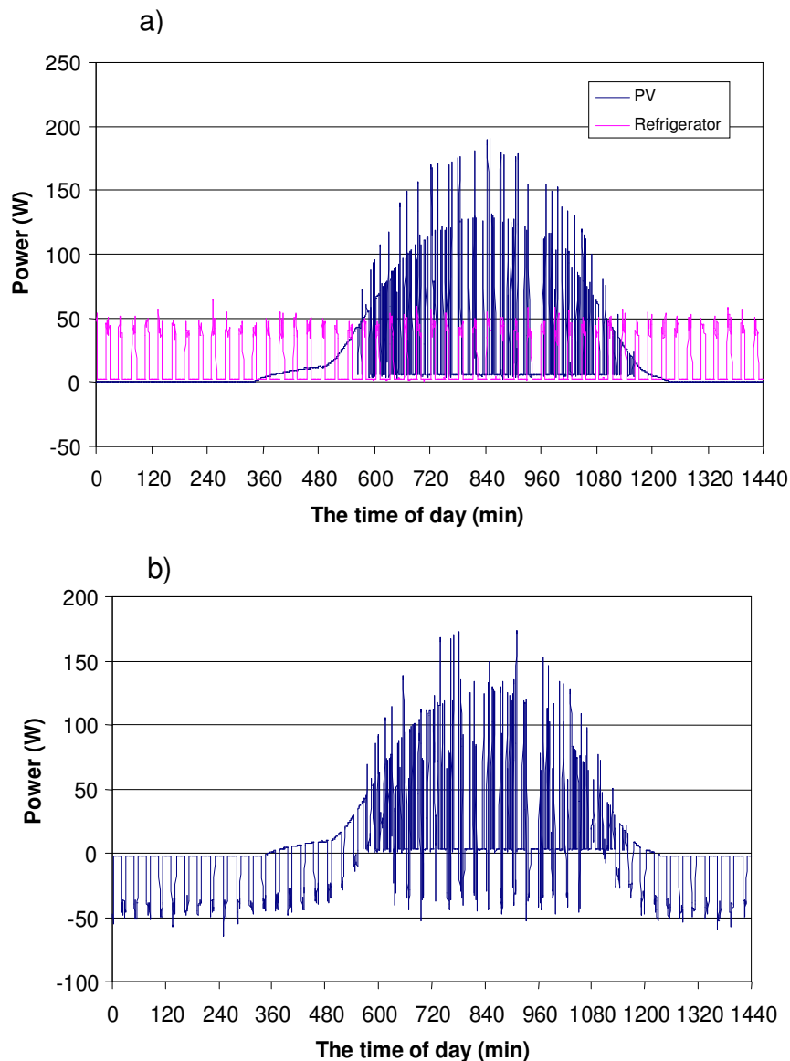
Figure 4. Instantaneous power values of the components for a typical hot day in May 2009, where t = 0 corresponds to local time of 8:00 AM; (a) PV and refrigerator, (b) battery-bank.
