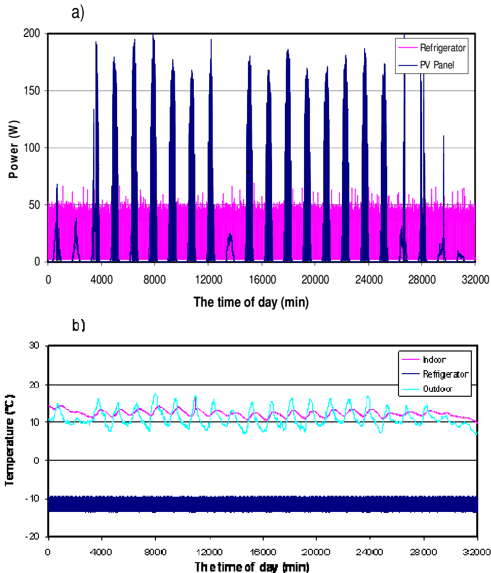
Figure 5. Long-term (during 23 days) behavior of the PV-refrigerator parameters during winter days in December 2009, where t = 0 corresponds to local time of 8:00 AM; (a) Corresponding powers of refrigerator and PV panel, (b) Corresponding temperatures of refrigerator-cabin, room-interior and the ambient.
