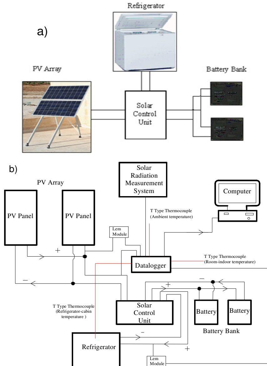
Figure 2. (a) Schematic of the PV-refrigerator system, (b) Experimental measurement loop.
