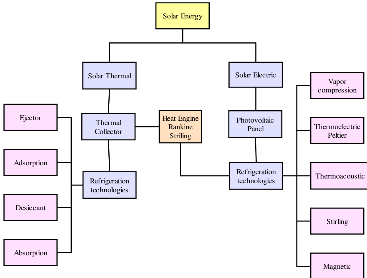
Figure 1. Classification of solar refrigeration systems (Kim and Ferreira, 2008; Papadopoulos et al., 2003; Ewert et al., 1998).
