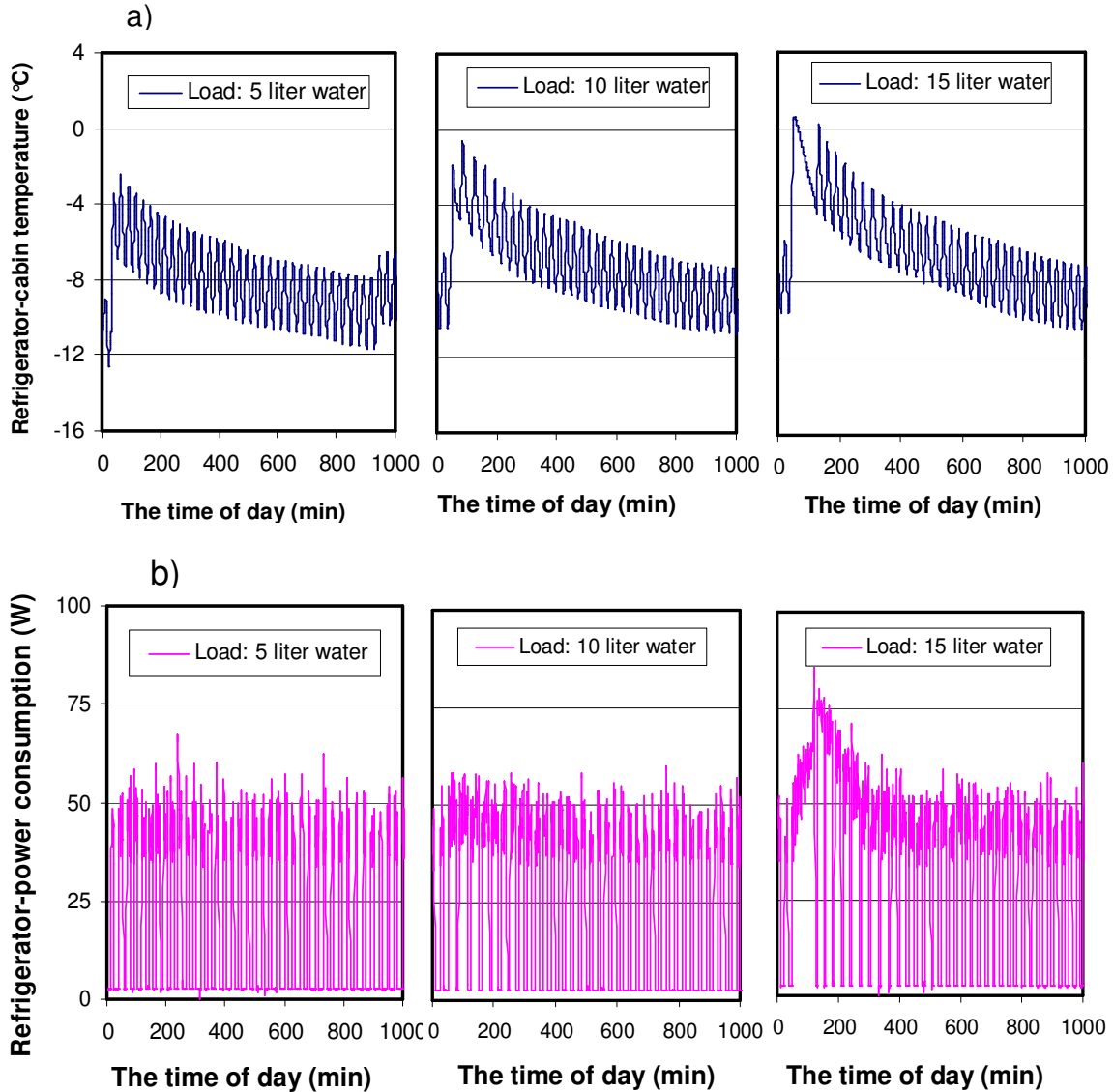
Figure 7. Relative effect of cooling load on instantaneous operating parameters of the PV-refrigerator under systematically increased cooling load condition for a typical hot day in May 2009, where t = 0 corresponds to local time of 8:00 AM; (a) refrigerator-cabin temperature, (b) refrigerator-power consumption.
