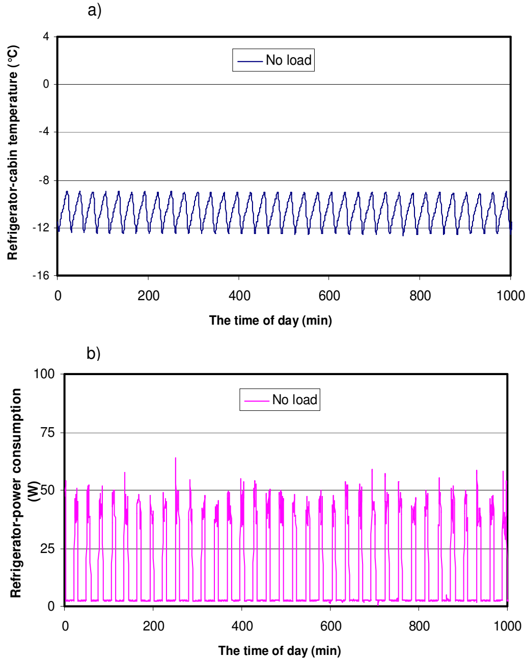
Figure 6. Typical behavior of instantaneous operating parameters of the PV-refrigerator under no-extra-cooling load condition for a typical hot day in May 2009, where t = 0 corresponds to local time of 8:00 AM; (a) refrigerator-cabin temperature, (b) refrigerator-power consumption.
