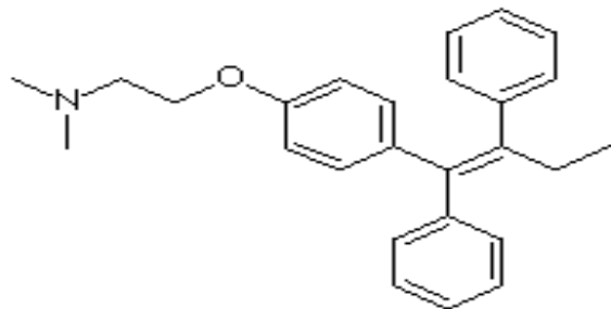
Figure 3. Tamoxifen.
