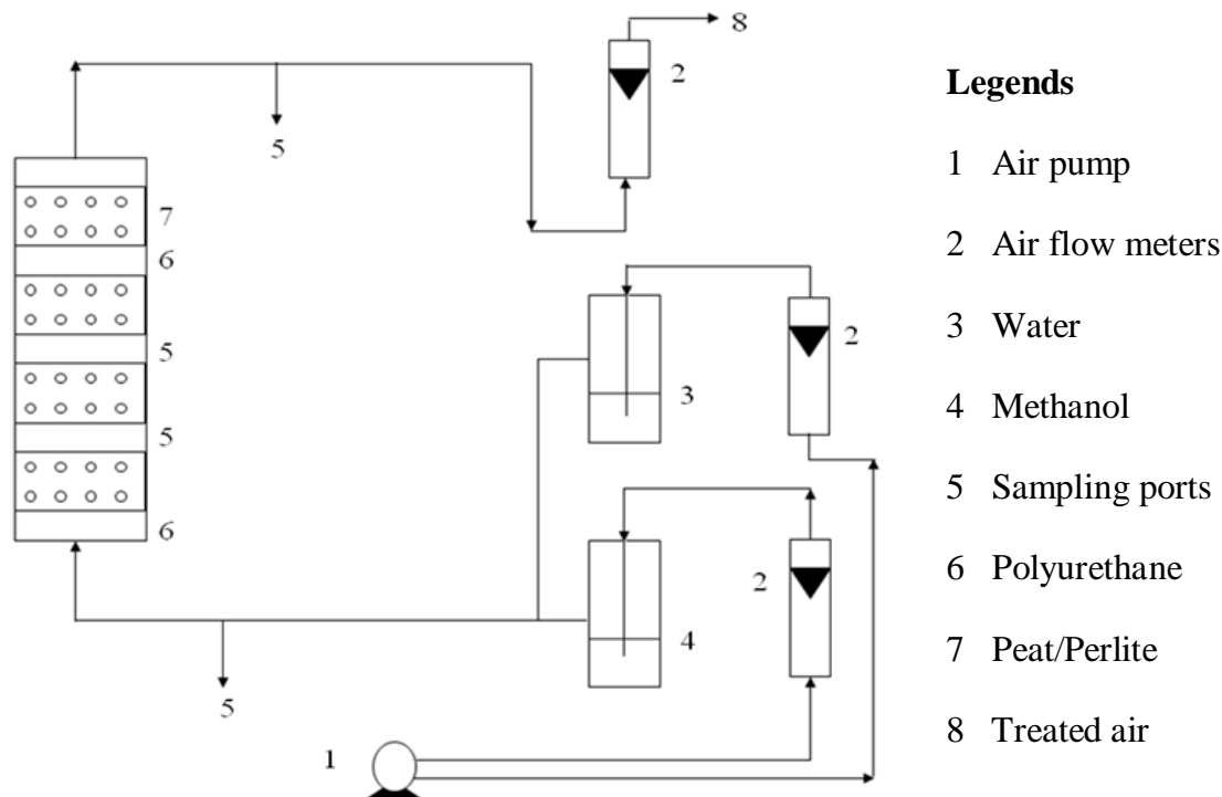
Figure 2. Schematic diagram of a closed type biofilter (Source: Bajpai et al., 1999).
