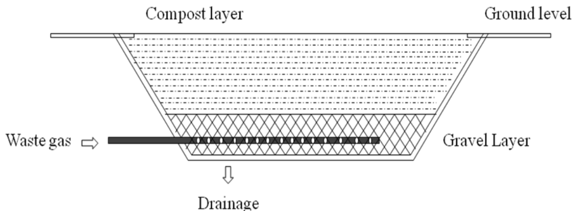
Figure 1. Cross-section of a conventional open type biofilter (Bajpai et al., 1999).
