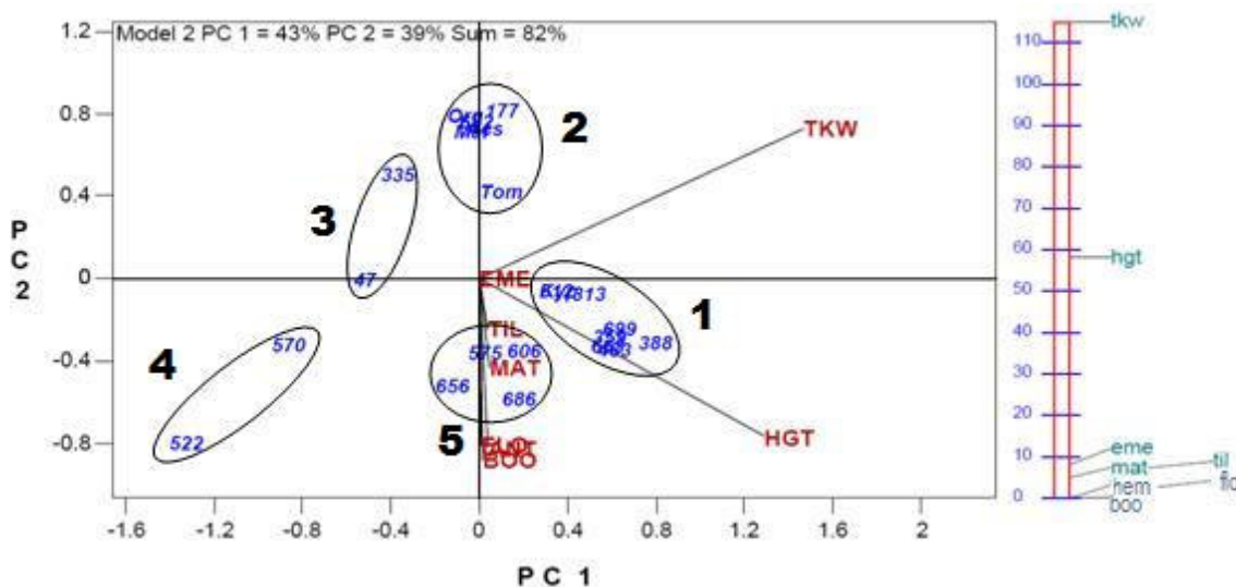
Figure 1. The durum wheat genotype by trait biplot based on 23 genotypes x 8 agromorphological traits two-way table. The numbers indicated in blue in figure denotes accessions number as indicated in Table 1. EME: days to emergence, TIL: days to tillering, BOO: days to booting, HEM: days to head emergence, FLO: days to flowering, MAT: days to physiological maturity, HGT: plant height and TKW: thousands kernel weight. PC1 and PC2 are the first and second principal components, respectively, accounting for 82% of total variance. Marked groups (1 - 5) are discussed in the text.
