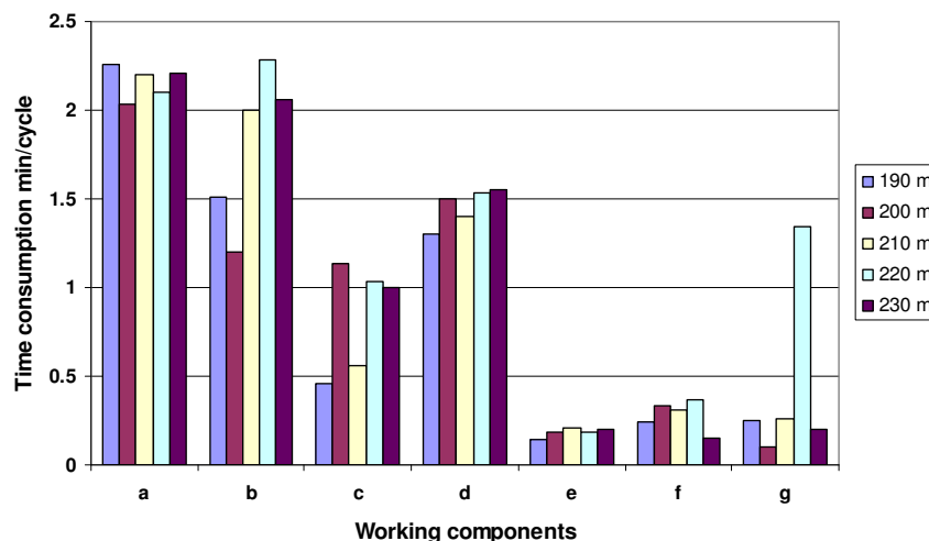
Figure 6. Time consumptions of working component.
