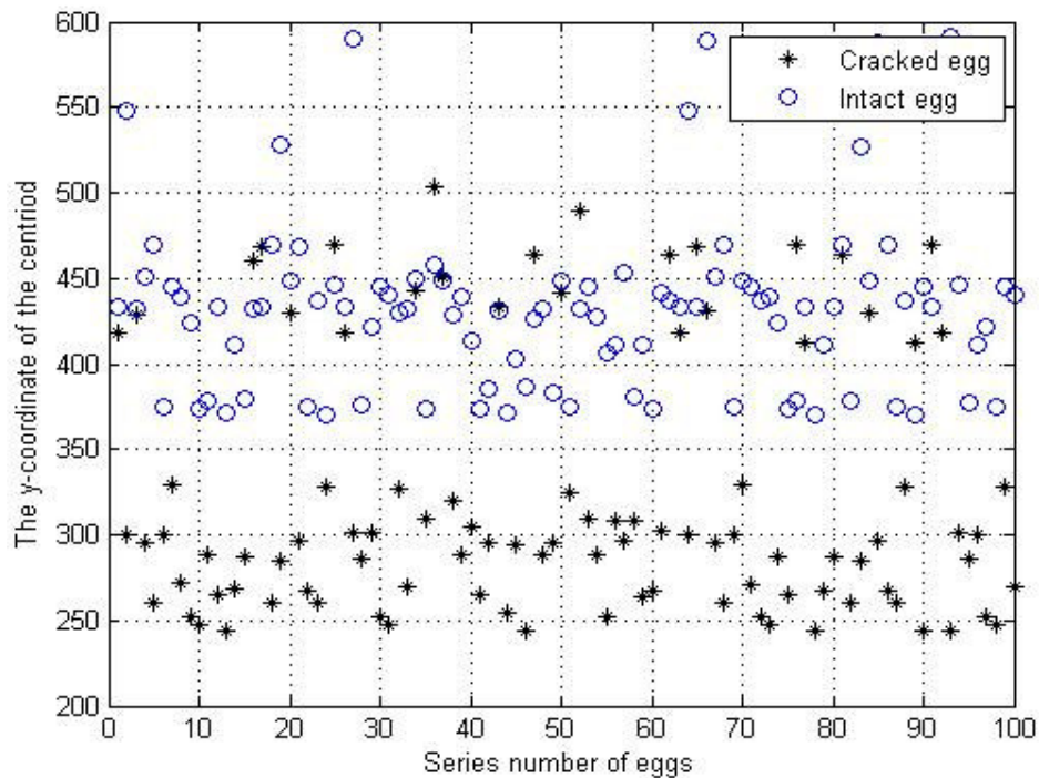
Figure 8. The distribution of y-coordinates of the frequency domain centroid for 100 intact eggs and 100 cracked eggs.
