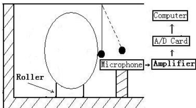
Figure 1. Schematic diagram of detection system.
