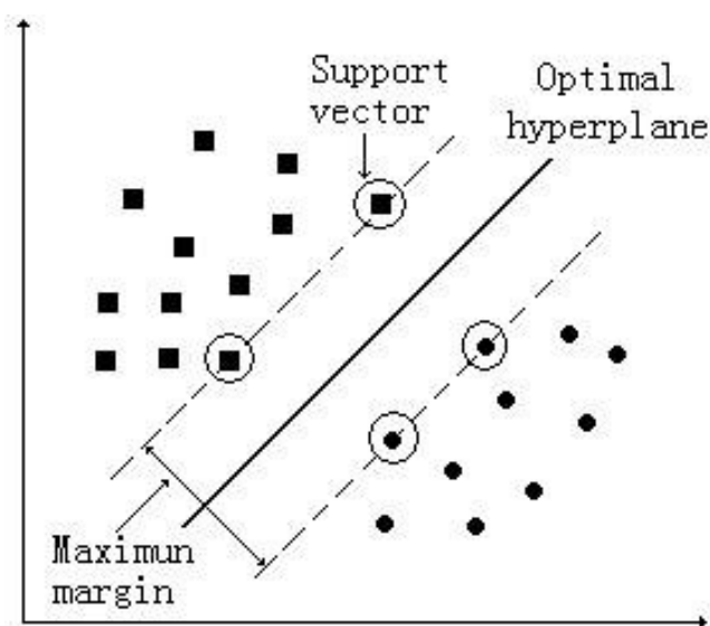
Figure 2. Maximum-margin hyper-plane for a SVM trained with samples from two classes.
