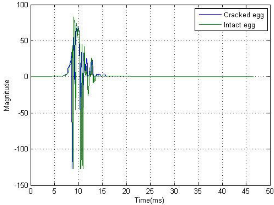
Figure 3. Typical time signal of the response of eggs.
