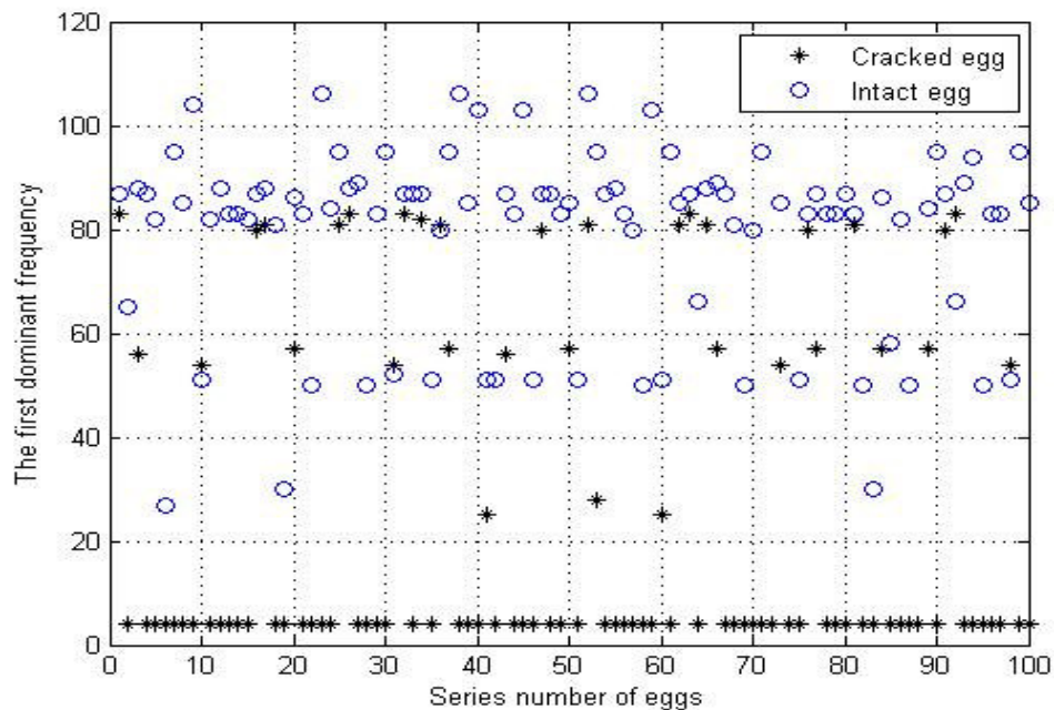
Figure 6. The distribution of the first dominant frequency for 100 intact eggs and 100 cracked eggs.
