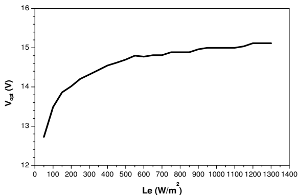
Figure 4. Simulation of the influence of solar radiation on the Vopt voltage of module SP75 at the temperature 25°C.
