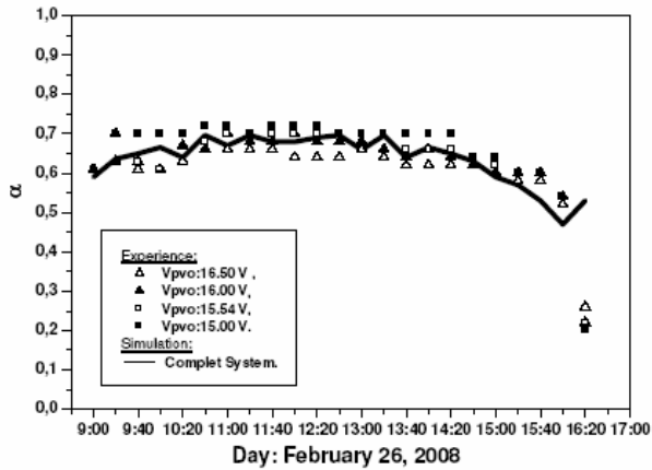
Figure 23. Variation of the duty cycle of PV system during the day February 26, 2008.
