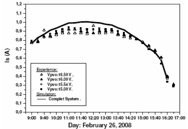
Figure 27. Variation of the Is current on the output of the DC-DC converter during the day February 26, 2008.
