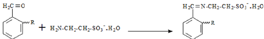
Figure 1. Synthetic schemes of taurine phenolic compound (TPC).
