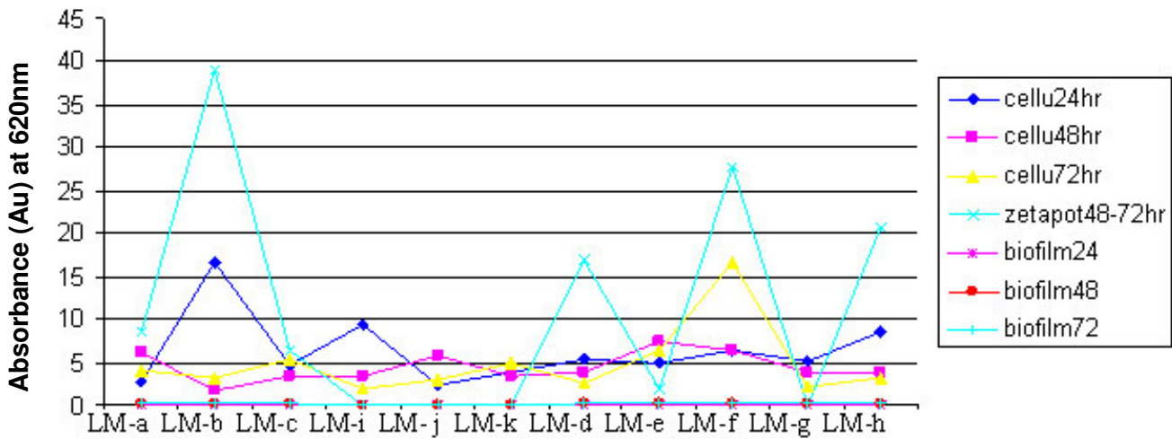
Virulence characteristics of L. monocytogenes -strains
