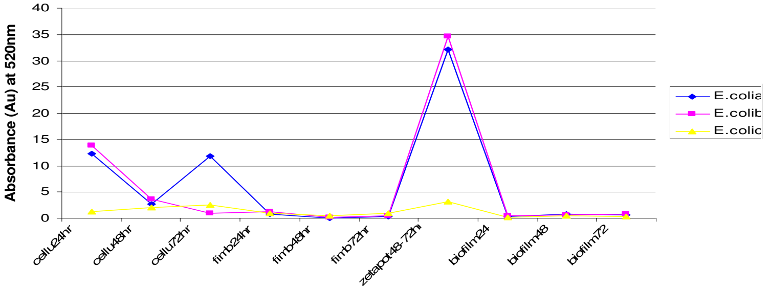
Virulence characteristics of E. coli O157H: 7 strains
