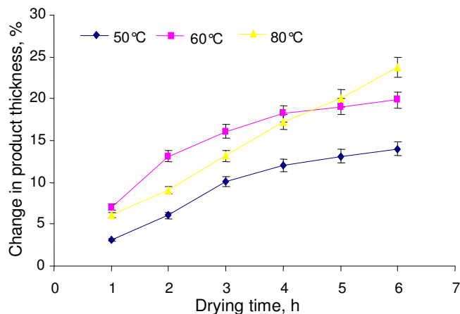
Figure 2a. Effect of drying temperature on change in product thickness of blanched banana slices.
