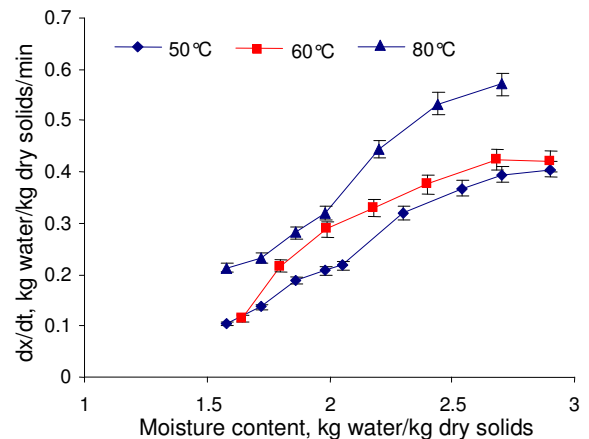
Figure 1c. Drying rate curves of blanched unripe banana at different temperatures.
