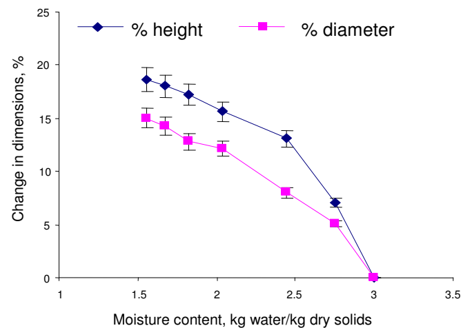
Figure 3c. Changes in product dimensions of ripe untreated banana samples dried at 60°C.
