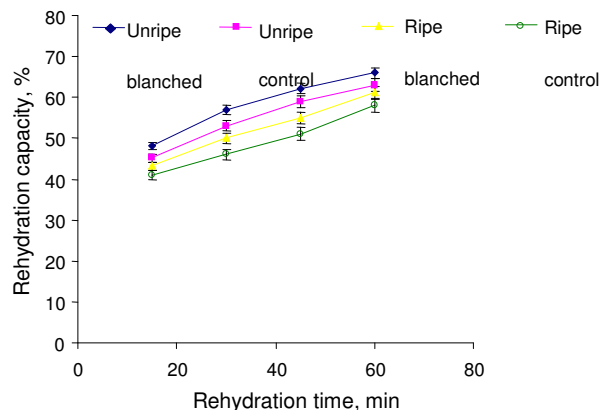
Figure 5b. Influence of blanching and ripeness on the rehydration capacity of banana Slices with rehydration time.
