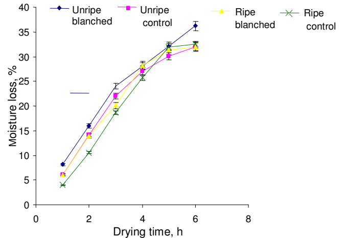
Figure 1b. Effects of blanching and ripening on moisture loss of banana slices dried at 50°C with time.
