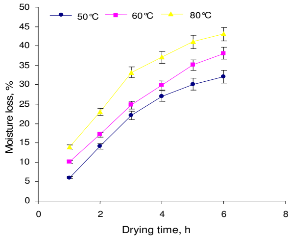
Figure 1a. Effect of drying temperature on percent moisture loss of untreated banana slices with time.
