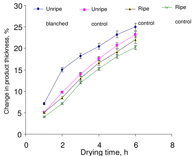
Figure 2b. Influence of blanching and ripeness on the change in product thickness of banana slices dried at 80°C.
