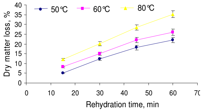
Figure 6a. Effect of drying temperature on dry matter loss with rehydration time of unripe banana slices.
