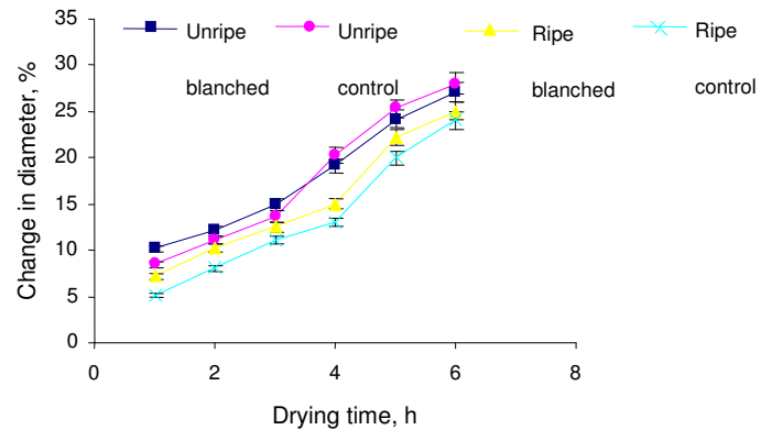
Figure 3b. Changes in product diameter of banana slices dried at 80°C.
