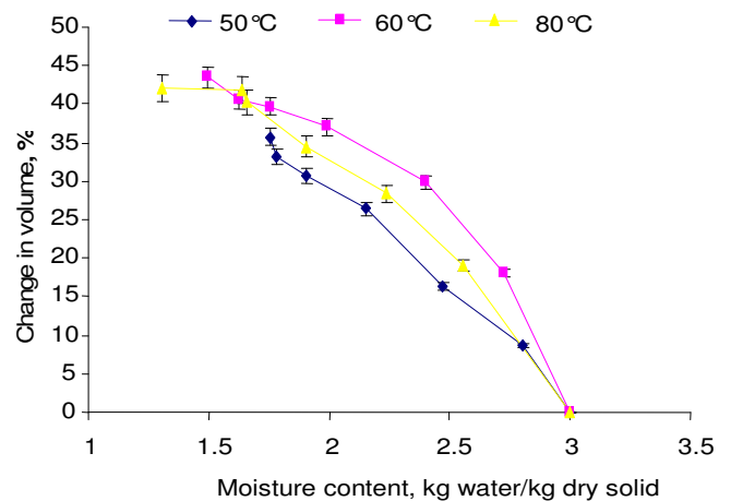
Figure 4b. Influence of moisture content and drying temperature on change in volume of ripe blanched banana samples.
