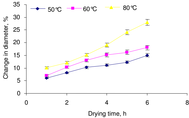
Figure 3a. Changes in diameter of ripe banana slices with drying temperature and time.
