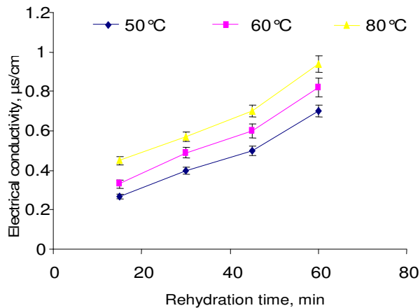
Figure 7a. Effect of drying temperature on electrical conductivity of immersion solution of unripe banana slices rehydrated with time.
