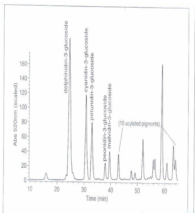
Figure 2. HPLC chromatogram of standard anthocyanins.
