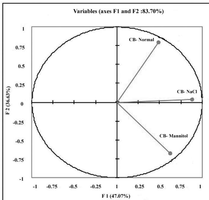
Figure 7. PCA plot generated for the three samples of C. borivilianum treated with stress conditions.
