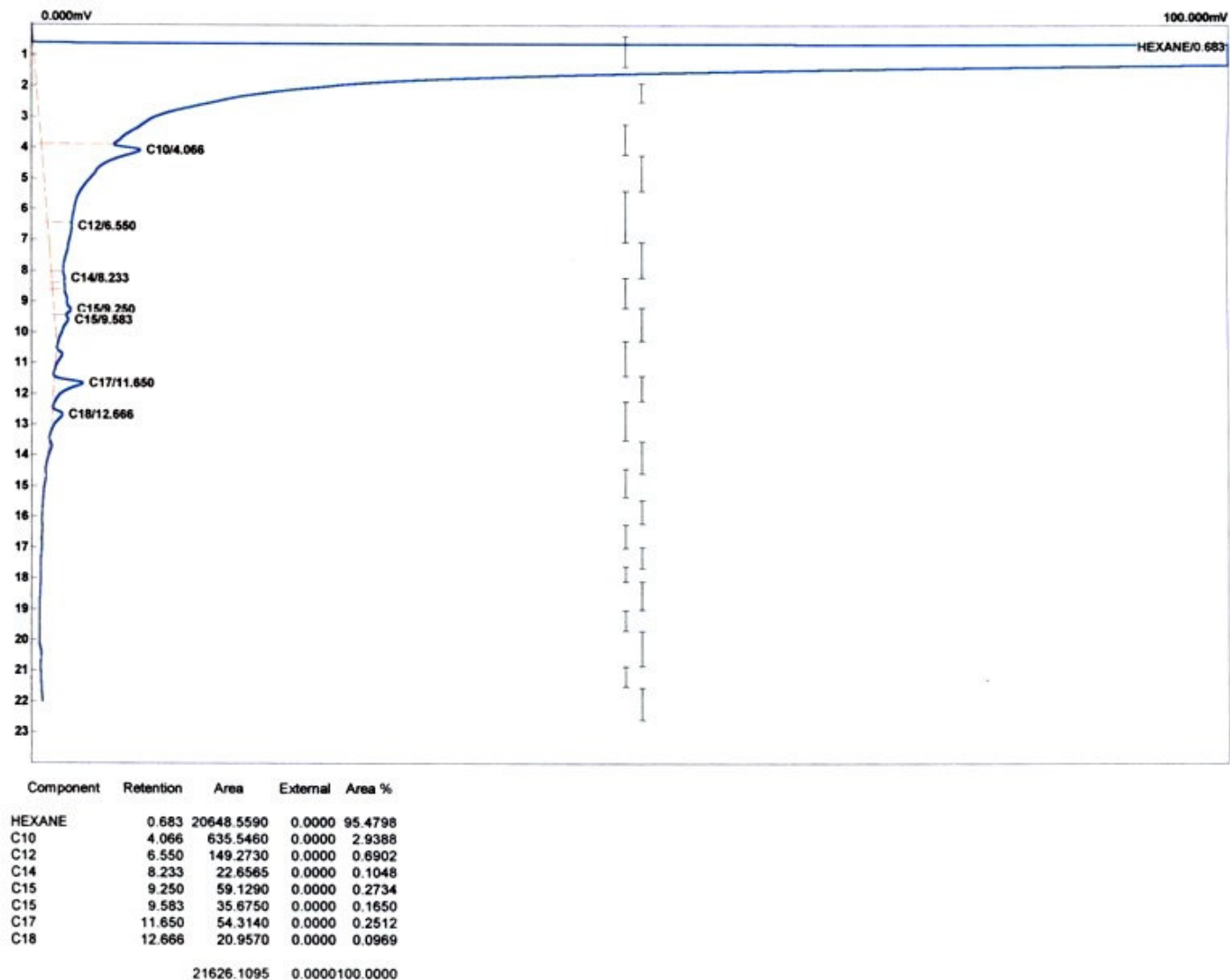
Figure 14. GC profile of detergent residues (shake flask experiment). AK 37 = ELEPHANT detergent.
