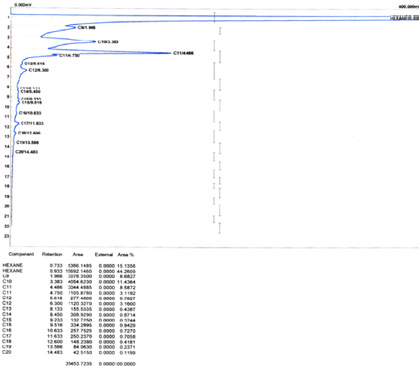
Figure 11. GC Profile of detergent residues (shake flask experiment). AK 67 = Sodium dodecyl sulphate (SDS).
