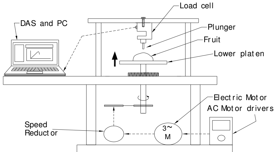
Figure 1. Measurement setup for ruptures properties.
