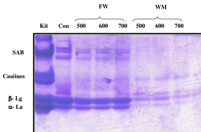
Figure 1c. SDS PAGE of milk (WM) and fresh whey treated (FW) by microwave irradiation at 500, 600 and 700 Watts during 10 min. Kit: Molecular weight Kit marker: bovin serum albumin (68 000 Da), caseine (24,000 Da), \beta -Lactoglobulin ( \beta - Lg, 18,000 Da), and \alpha -Lactalbumin ( \alpha - La, 14,000 Da). Control: fresh whey no treated.
