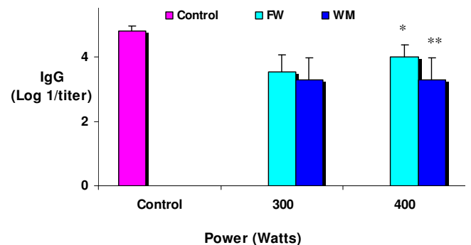
Figure 2b. Binding ability (antigenicity) of \beta -Lg rabbit IgG to fresh whey (FW) and whey descended from whole milk (WM) samples irradiated by microwave at 300,400 Watts during 15 minutes determined by ELISA. Values are given as mean \pm SE (standard error) from independent measurements (n=6). (* : 0,01 < p < 0,05 ; ** : p < 0,01 ; *** : p < 0,001)
