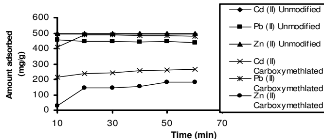
Figure 7. Amounts adsorbed against time (min) for Cd (II), Pb (II) and Zn ions on unmodified and carboxylated maize cob of 425 \mu m particle size. (Initial concentration is 1000 mg/l).
