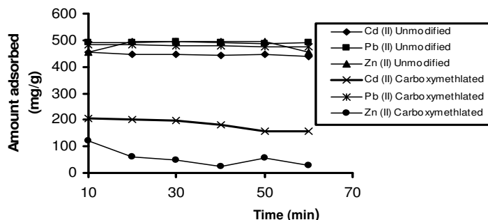
Figure 6. Amount adsorbed (mg/g) against time (min) for Cd (II). Pb (II) and Zn (II) ions on unmodified and carboxylated maize husk of 425 \mu m particle size. (Initial concentration is 1000 mg/l).
