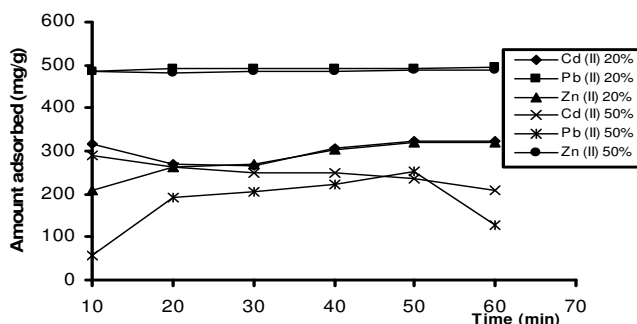
Figure 3. Amount adsorbed (mg/g) against time (min) for Cd (II), Pb (II) and Zn (II) ions on maize cobs of 425 \mu\text{m} particle size effect of 20% and 50% isopropanol (Initial metal ion concentration is 1000 mg/l).
