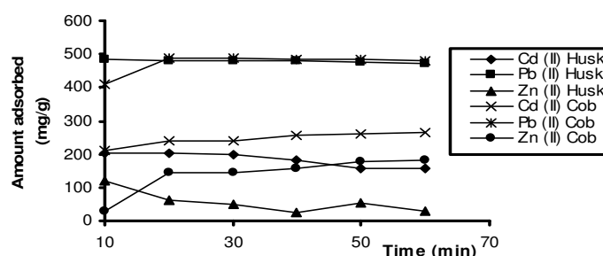
Figure 5. Amount adsorbed (mg/g) against time (min) for Cd (II), Pb (II) and Zn (II) ions on carboxymethylated maize cob and husk of 425 \mu m particle size. (Initial concentration is 1000 mg/l).
